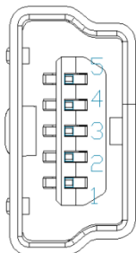
Figure 15: Mass Storage USB Connector
