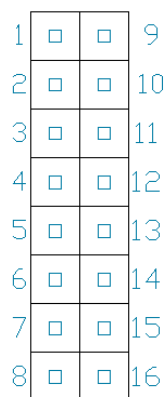
Figure 16: GPO Header
