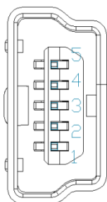
Figure 15: Mass Storage USB Connector
