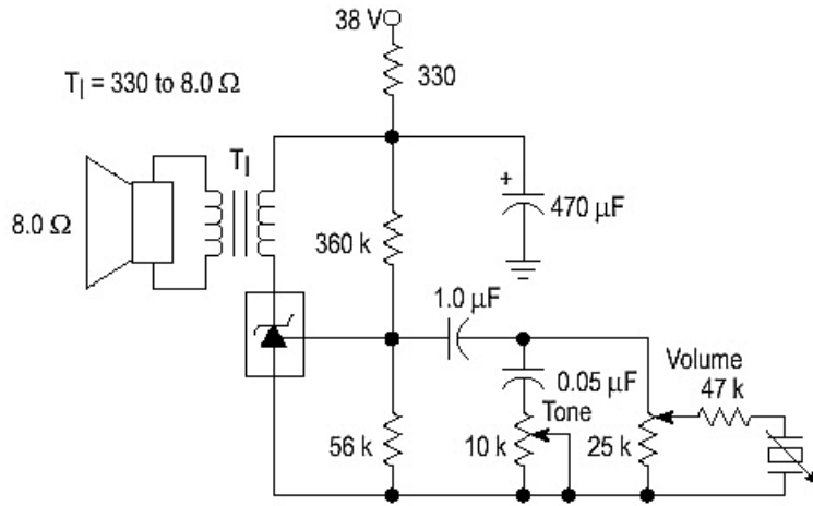
Fig 16 .Simple 400mW phone amplifier
