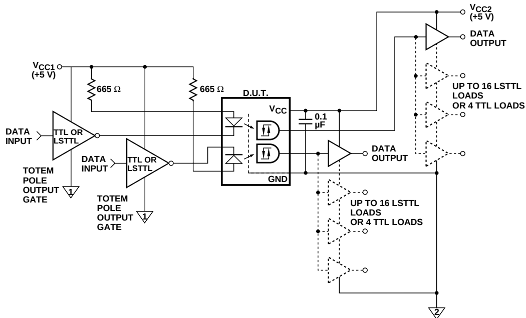
Figure 13. Recommended LSTTL to LSTTL Circuit.
