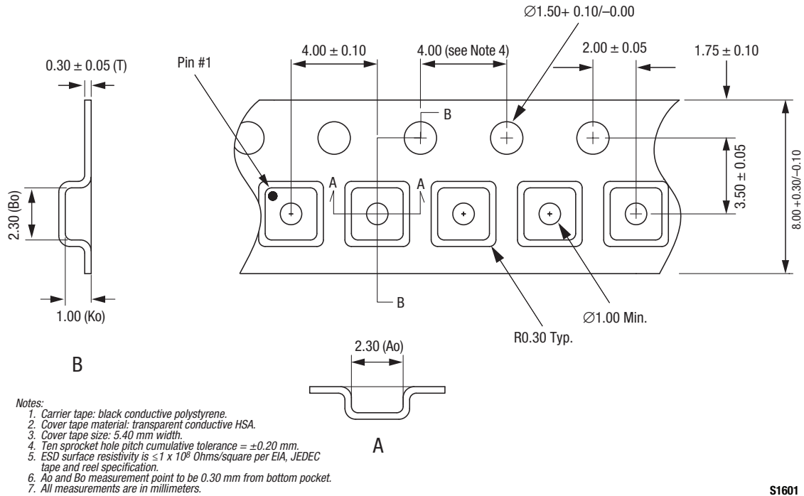
Figure 10. CLA4611-085LF Tape and Reel Dimensions
