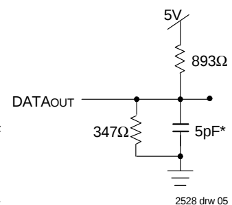
Figure 2. Output Test Load (for t_{HZ} , t_{WZ} , and t_{OW} )
