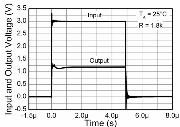
Pulse Response
