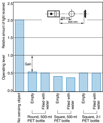
Dark Excess Gain vs. Sensing Object Characteristics
