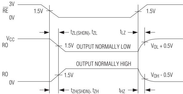
Figure 15. Receiver Enable and Disable Times (except MAX488E and MAX490E)
