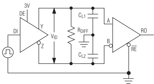
Figure 10. Driver/Receiver Timing Test Circuit
