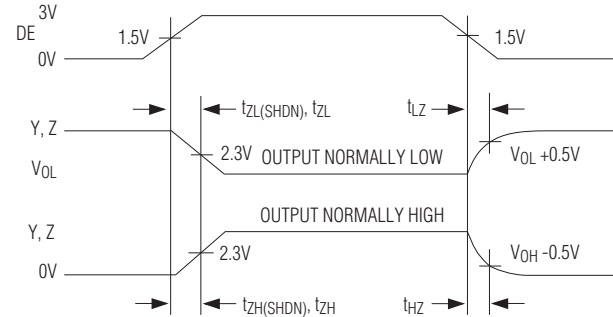
Figure 13. Driver Enable and Disable Times (except MAX488E and MAX490E)
