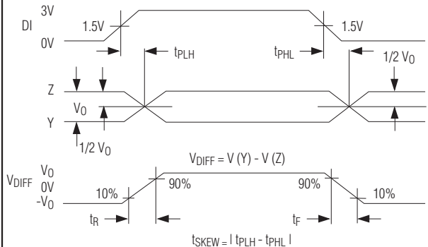
Figure 12. Driver Propagation Delays
