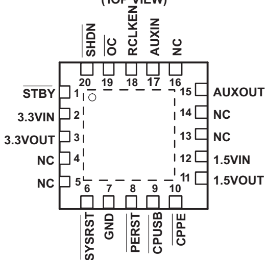
TPS2231 RGP PACKAGE (TOP VIEW)
