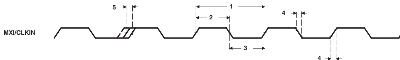
Figure 6-14. MXI/CLKIN Timing
