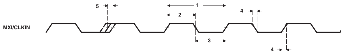
Figure 6-15. M24XI Timing
