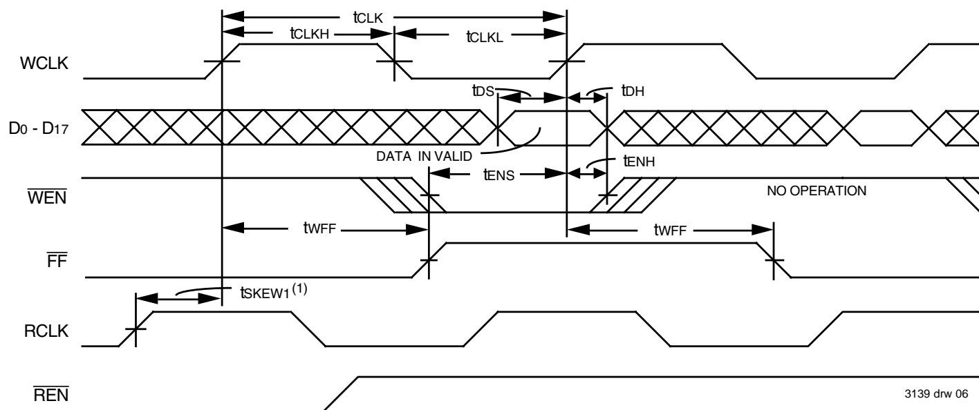
Figure 5. Reset Timing (2)
