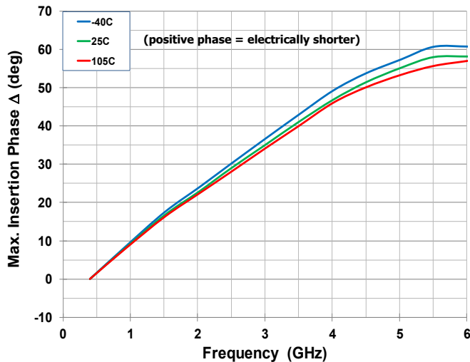
Max. Insertion Phase \Delta vs. Frequency
