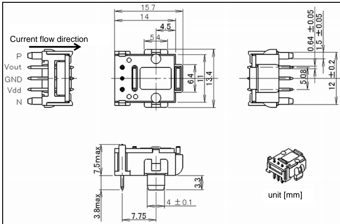
Fig.6-1 Dimensions
