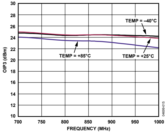
Figure 15. Output IP3 vs. Frequency and Temperature, Maximum Gain, I Only
