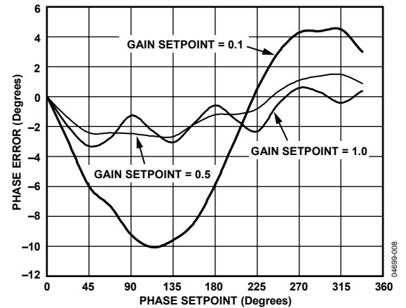
Figure 8. Phase Error vs. Phase Setpoint at Different Gain Setpoints
