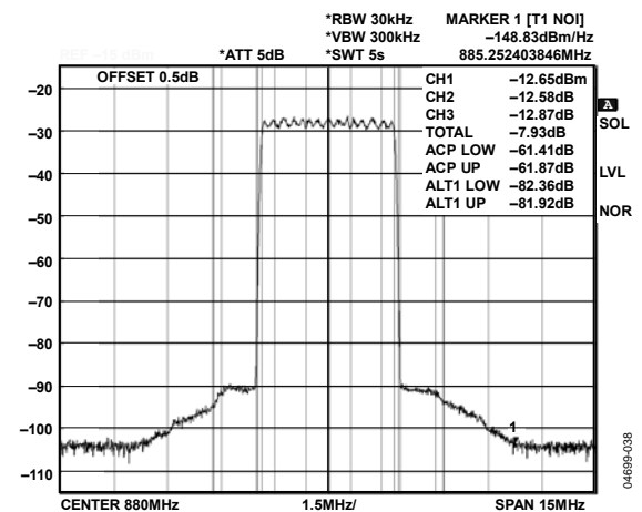
Figure 38. Output Spectrum, 3-Carrier CDMA2000 Test Model at -12.5 dBm/Carrier, V_i = V_Q = 0.353 V, ACP Measured at 2 MHz and 3.23 kHz Offset from Center of Spectrum, Noise Measured at 5.25 MHz Carrier Offset, Input Signal Filtered Using a Cavity-Tuned Filter (Pass Band = 4.6 MHz)
