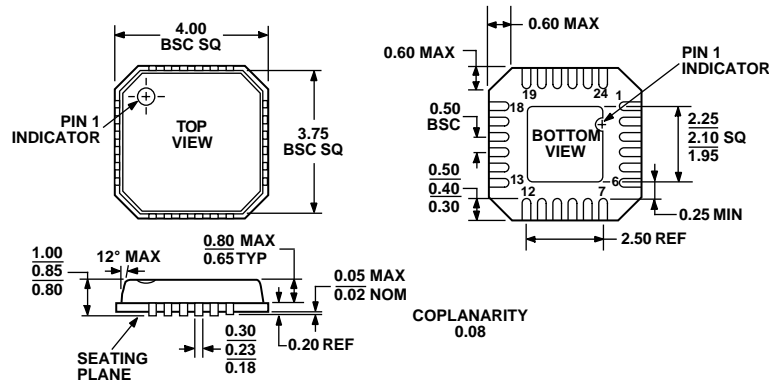
COMPLIANT TO JEDEC STANDARDS MO-220-VGGD-2 Figure 42. 24-Lead Lead Frame Chip Scale Package [LFCSP_VQ] 4 mm × 4 mm Body, Very Thin Quad (CP-24-1) Dimensions shown in millimeters
