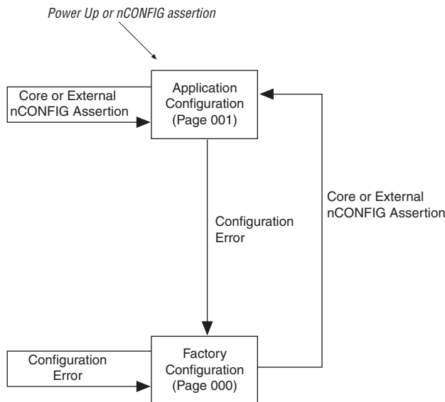
Figure 8–5. Transitions Between Configurations in Local Update Mode
