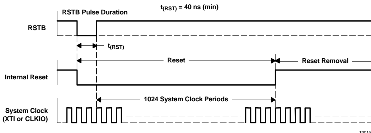
Figure 27. External Forced-Reset Timing
