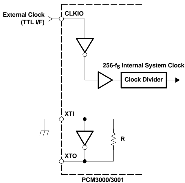
External Clock Input 2 : (XTO is open)
