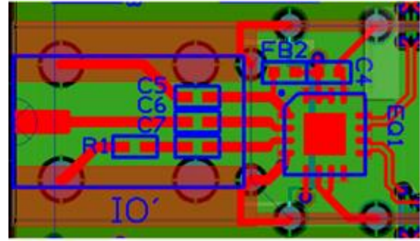
Figure 10: Recommended Layout
