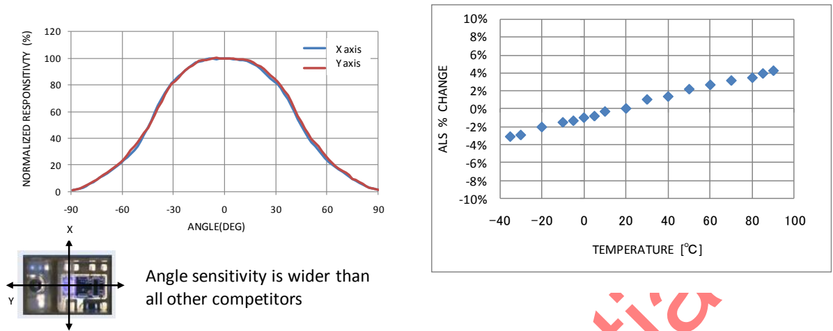
Figure 7 Ambient Light Sensitivity
