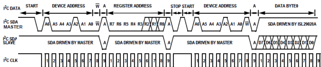
Figure 10 I 2 C DRIVER TIMING DIAGRAM FOR MASTER AND SLAVE CONNECTED TO COMMON BUS
