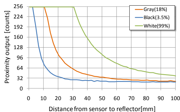
Figure 6 Proximity Sensitivity by color target
