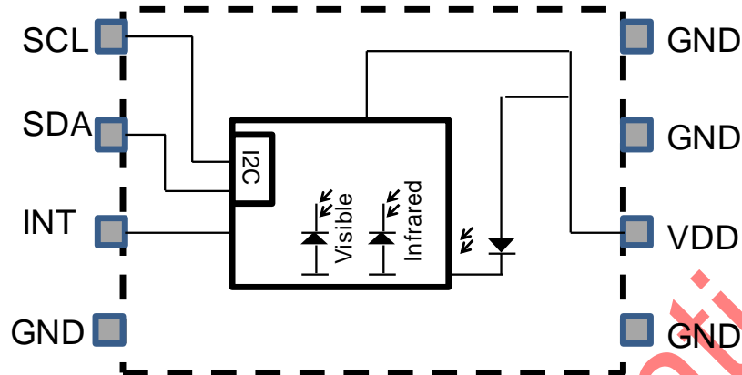
Figure 2 Function block diagram
