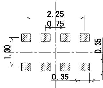
Figure 13 Recommended Land and Metal Mask pattern
