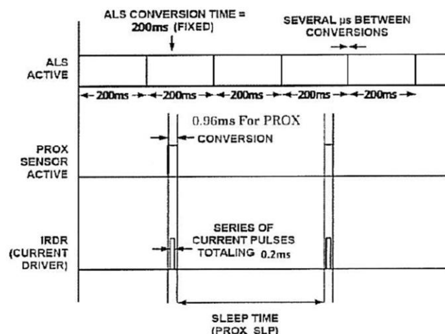
Figure 11 TIMING DIAGRAM FOR PROX/ALS EVENTS NOT TO SCALE
