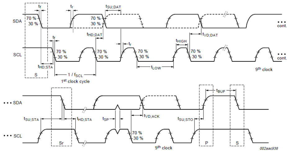
Figure 4 I2C TIMING DIAGRAM
