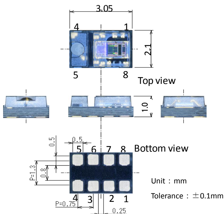
Figure 1 Outline Dimensions
