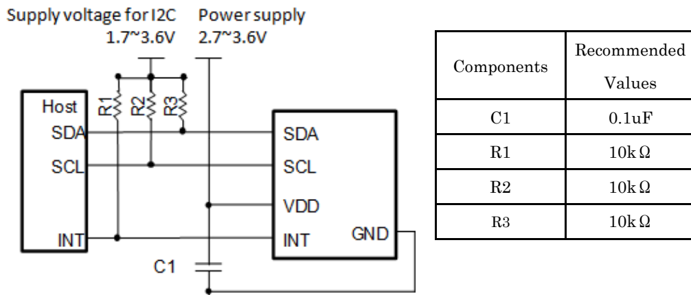
Figure 3 Recommended external circuit
