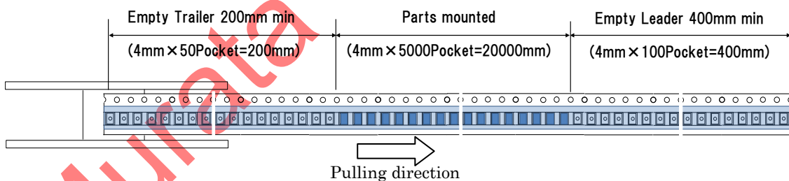
Figure 16 Pulling direction and Trailer/Leader
