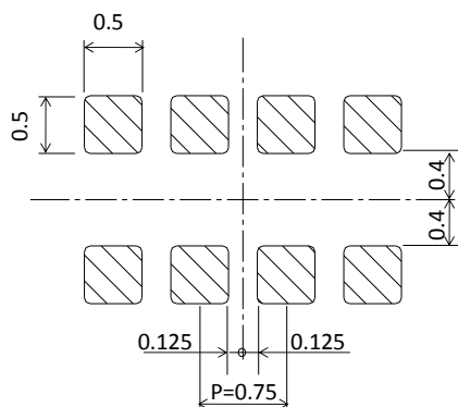
Figure 13 Recommended Land and Metal Mask pattern
