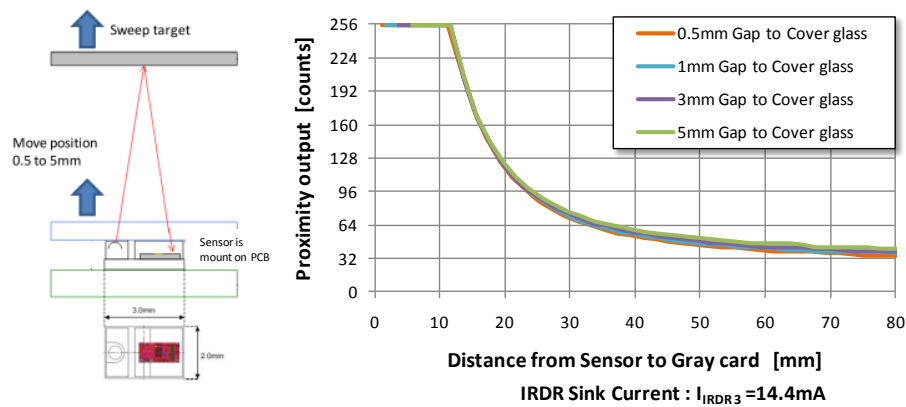
Figure 5 Proximity Sensitivity by cover glass
