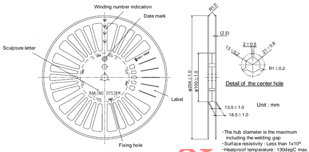
Figure 17 Reel structure and Dimensions
