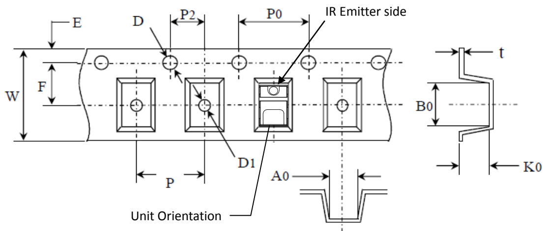
Figure 15 Tape dimensions and Product insertion
