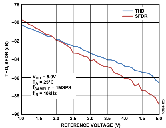
Figure 22. THD and SFDR vs. Reference Voltage
