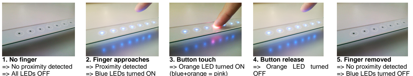
Figure 52 Touch+Proximity Module Operation
