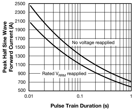
Fig. 4 - Maximum Non-Repetitive Surge Current Per Leg
