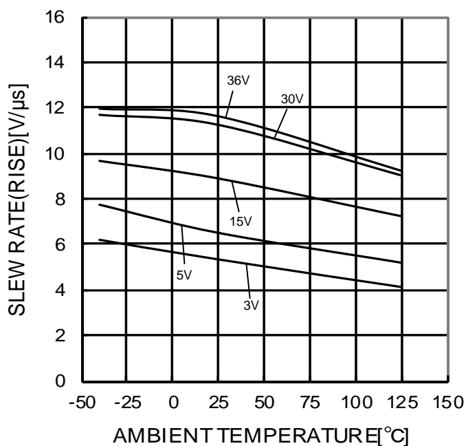
Figure 21. Slew Rate L-H Ambient Temperature (RL=10kΩ)
