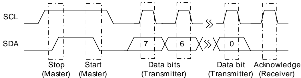
Figure 3. Data Transfer Protocol
