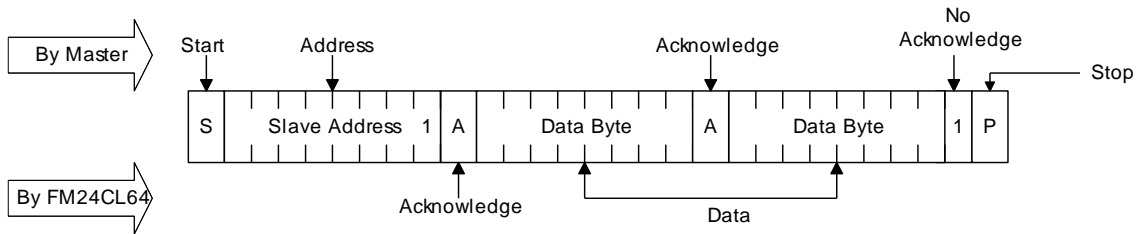
Figure 8. Sequential Read
