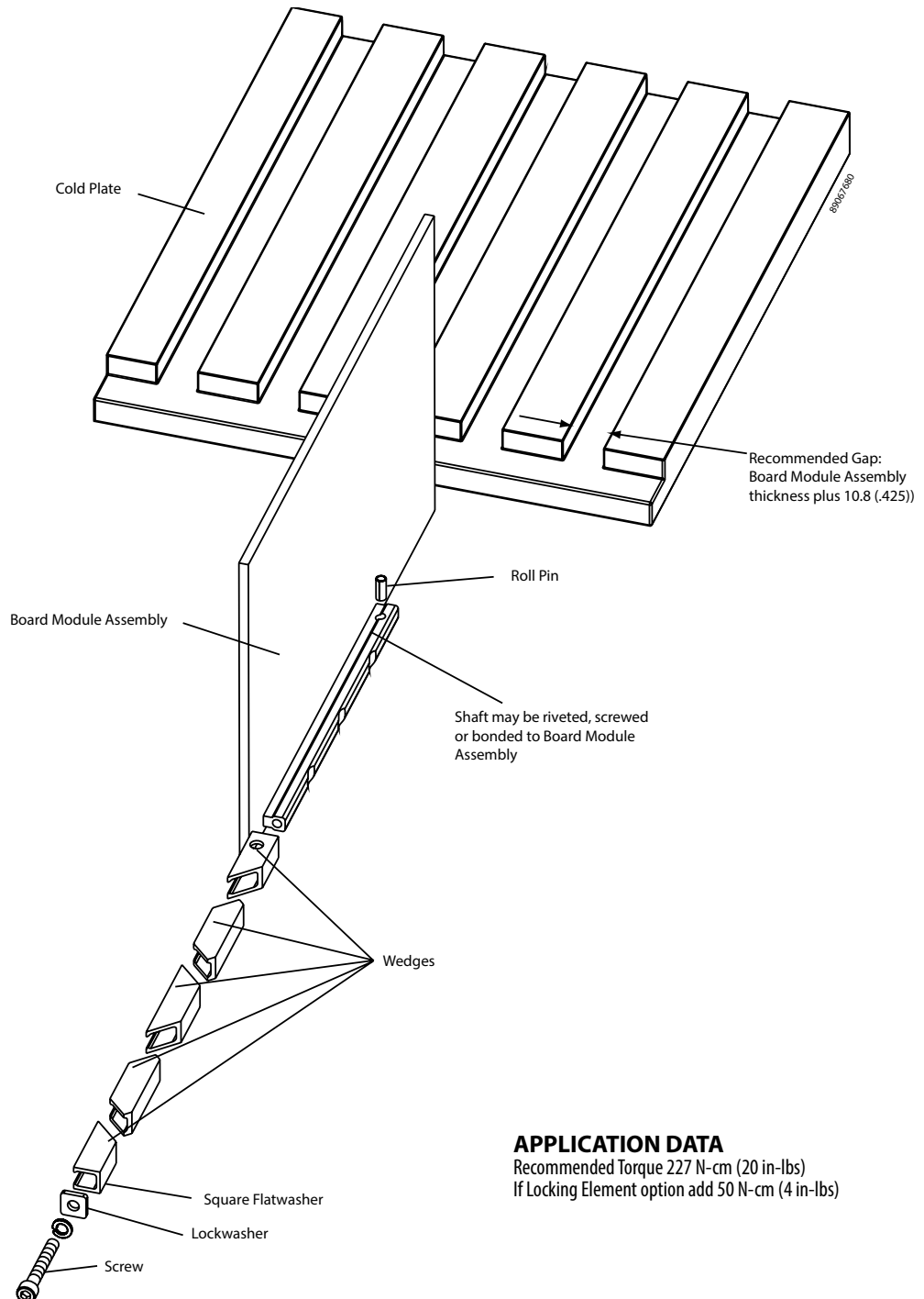
Series 280 - "Card-Lok" Retainer (Cold Plate)
