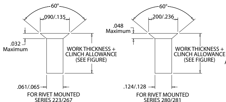
SUGGESTED RIVET DIMENSIONS
