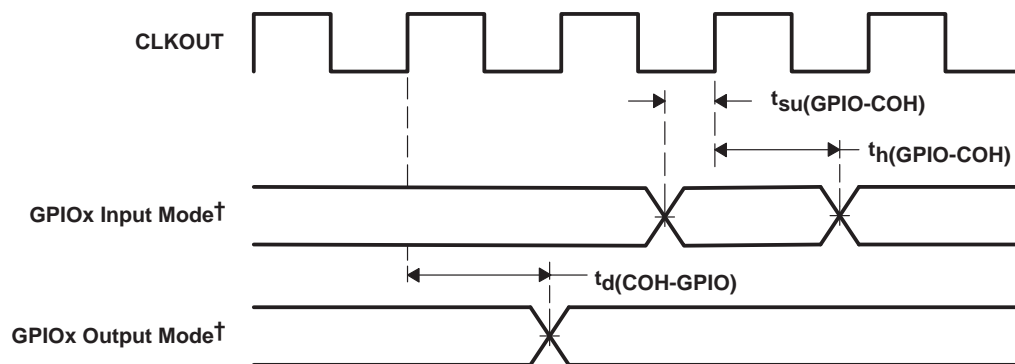
Figure 38. GPIOx † Timings
