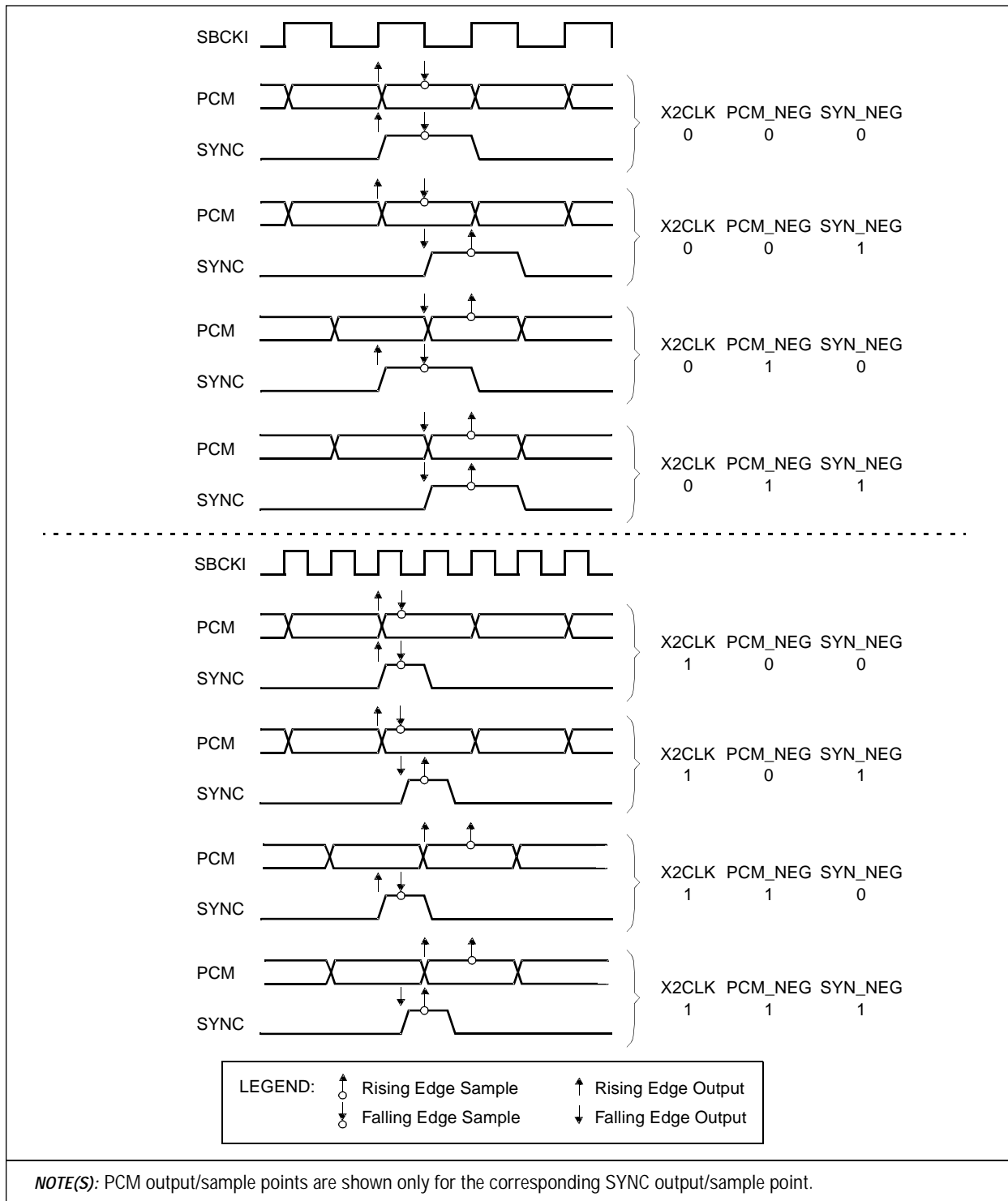
Figure 4-21. SBI Timing—Eight Clock Edge Combinations (Applicable to Any SBI Mode)
