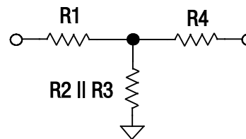
Figure 10. Simplified Circuit Topology (1 – 5 dB Attenuators)
