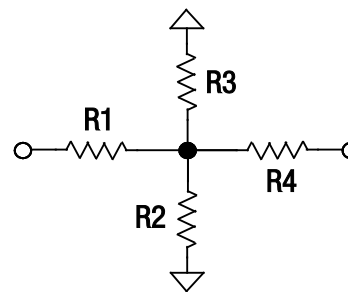
Figure 9. Circuit Topology (1 – 5 dB Attenuators)
