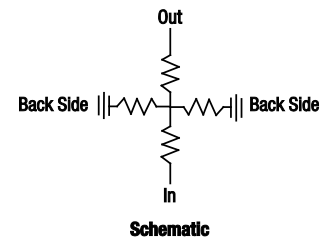
Figure 1. Typical Attenuator Die and Circuit
