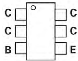
Pin-Out Top
