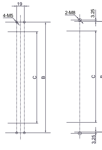
Mounting screw holes
