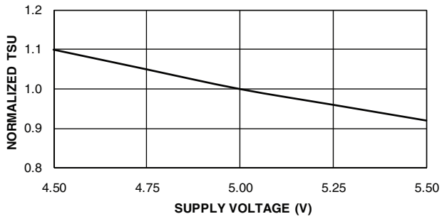
ATMEL ATF22V10C/CQ NORMALIZED T_{SU} VS. V_{CC}
