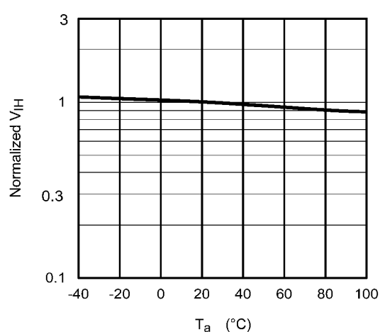
Fig. 12.10 Normalized V_H - T_a
