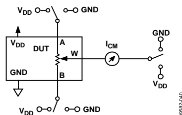
Figure 40. Common-Mode Leakage Current
