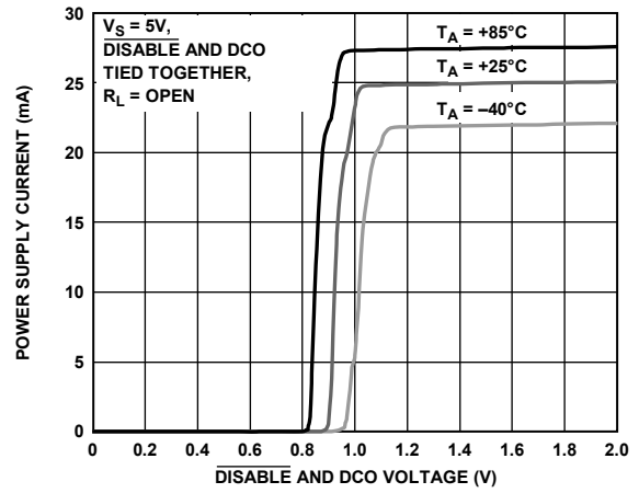
Figure 24. Supply Current vs. \overline{DISABLE}/DCO Voltage and Temperature
