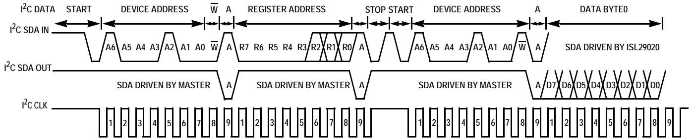
FIGURE 1. I²C READ TIMING DIAGRAM SAMPLE
