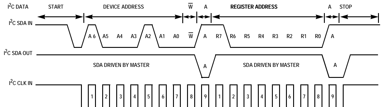
FIGURE 3. I²C SYNC_I²C TIMING DIAGRAM SAMPLE
