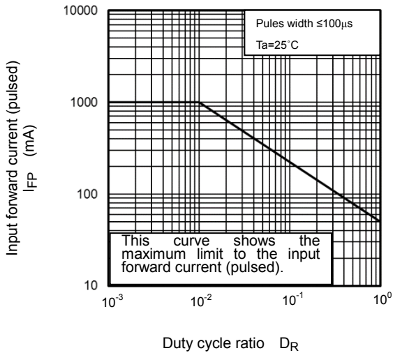
I_{FP} - D_R
