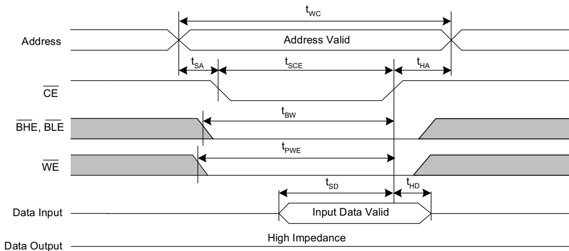
Figure 10. SRAM Write Cycle 2: \overline{\text{CE}} Controlled [3, 19, 20, 21]
