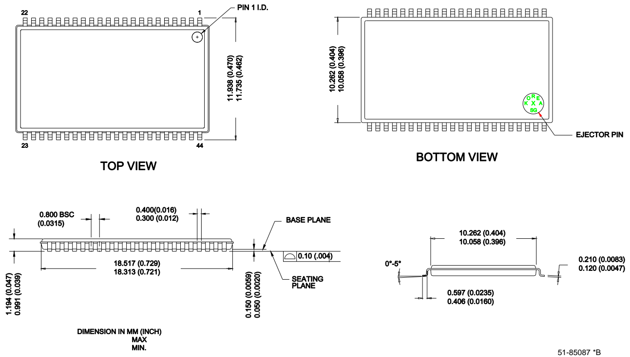
Figure 17. 44-Pin TSOP II (51-85087)
