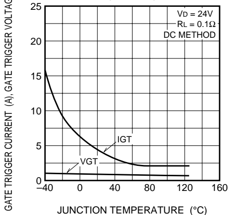
GATE TRIGGER CURRENT, GATE TRIGGER VOLTAGE VS. JUNCTION TEMPERATURE (TYPICAL)
