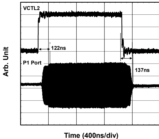
Switching Time
