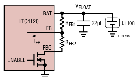
Figure 6. Programming the Float Voltage with the LTC4120
