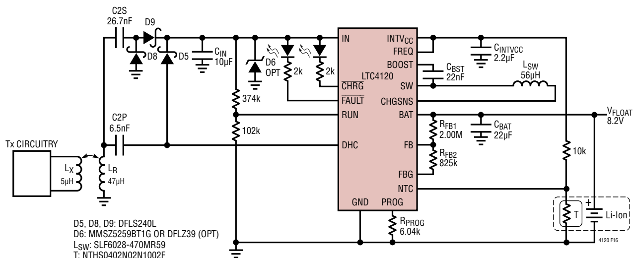
Figure 16. Resonant Coupled Power Transfer Charger Application
