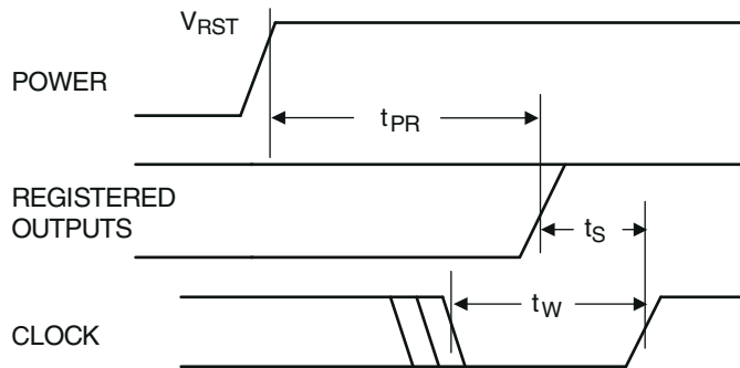
Figure 7-1. Programming/Erasing Timing
