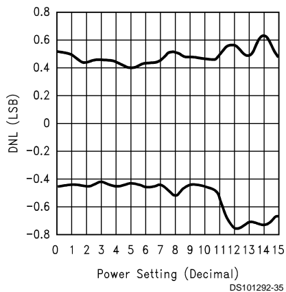
DNL vs. Power Setting @ 27 MHz Clock Frequency
