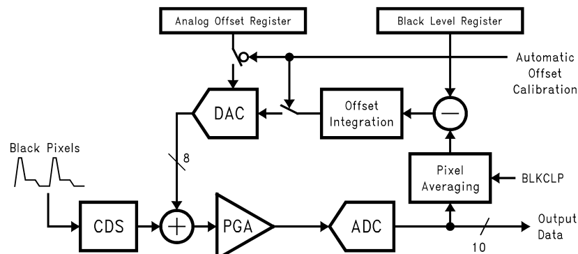
FIGURE 10. Digital Black Level Correction Loop
