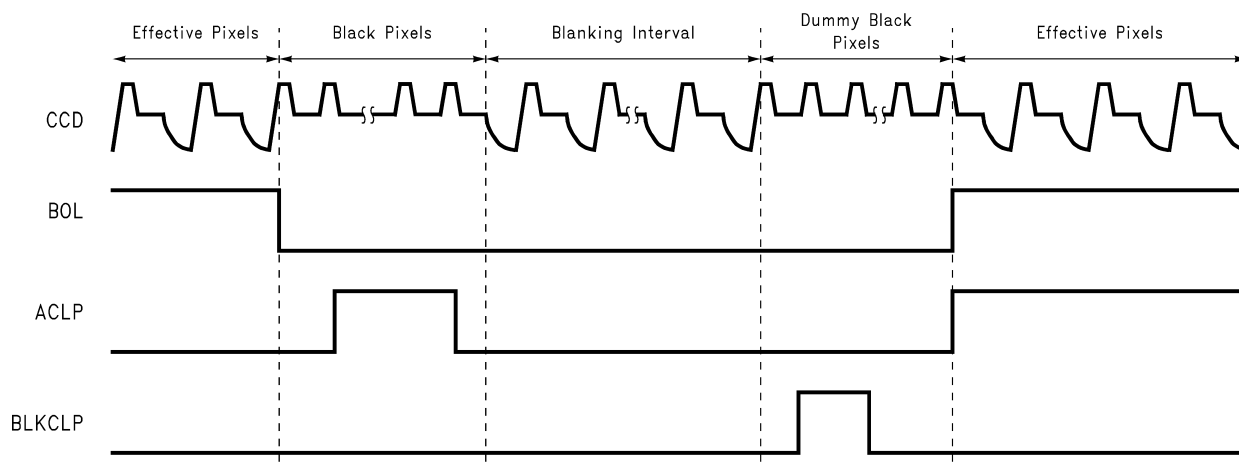
FIGURE 6. Typical Horizontal Interval Timing
