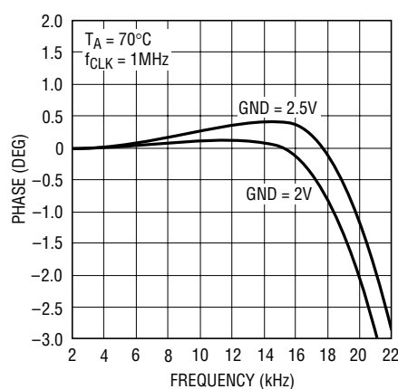
Maximum Passband for Single 5V, 50:1, for Two Ground Bias Levels
