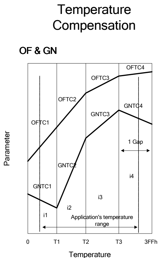
Figure 2. Temperature Compensation.
