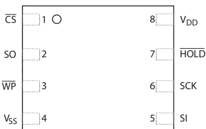
8-Pin DFN or 8-Pin DFN Small Flag Package
