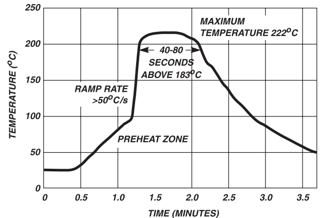
FIGURE 7. VAPOR PHASE SOLDER PROFILE
