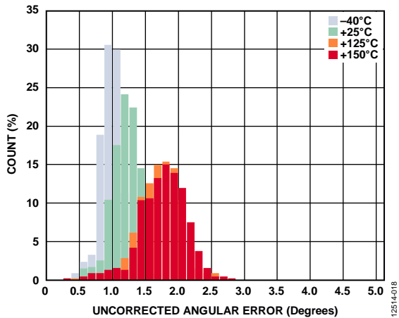
Figure 11. Uncorrected Angular Error, V_{DD} = 2.7\text{ V} , GC = \text{On}
