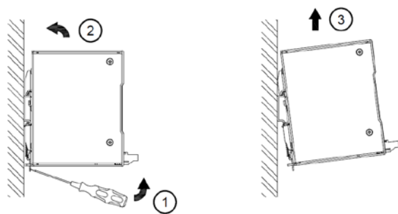
Fig. 2.2 Dismounting
